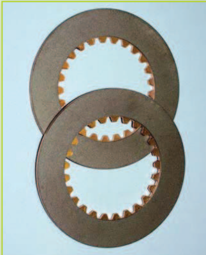
FRICTION PLATE D83xD55x3 S3
