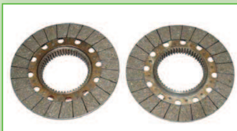
CLUTCH PLATE LOKOTRAKTOR D360xD240x4 HDS-57
